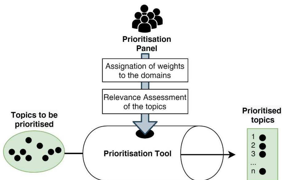
Figure 3. Prioritisation process
