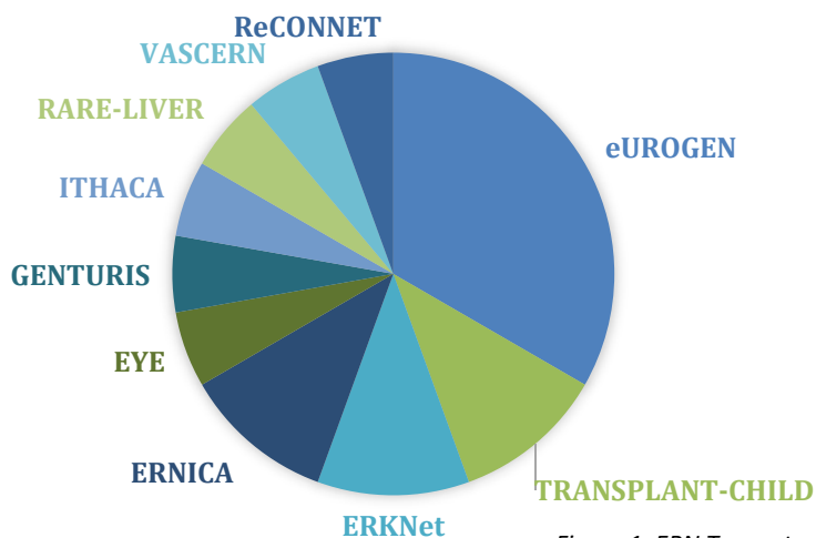
Figure 1. ERN Turnout
