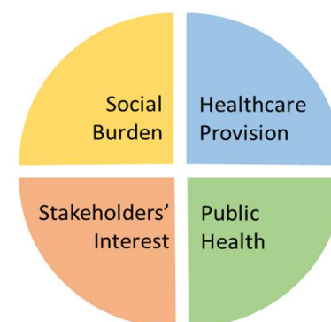
Figure 2. Prioritisation domains
